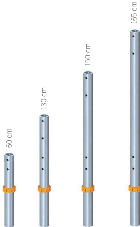
CONSOLE POSTS
